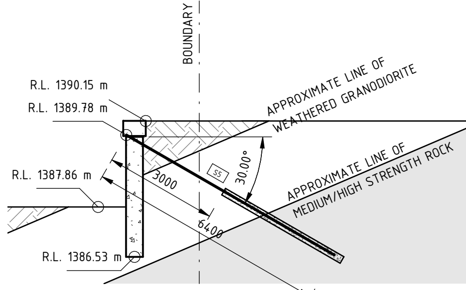
PILE S5
