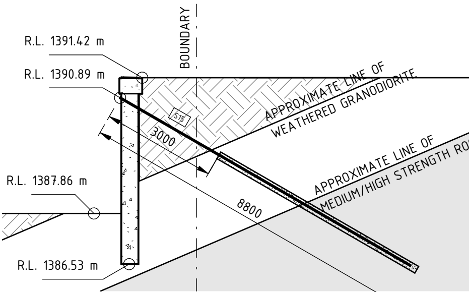
PILE S15
