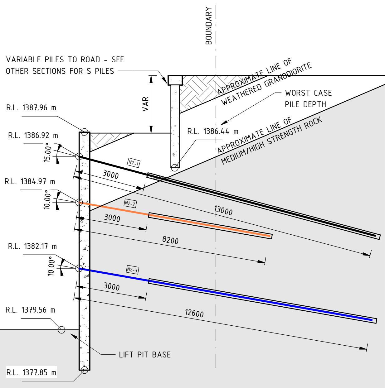
PILES N2
