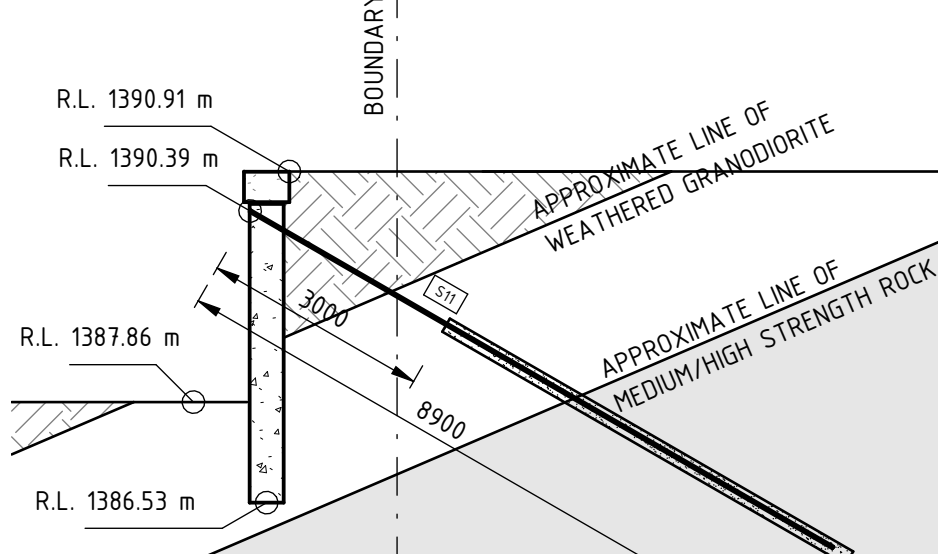
PILE S11
