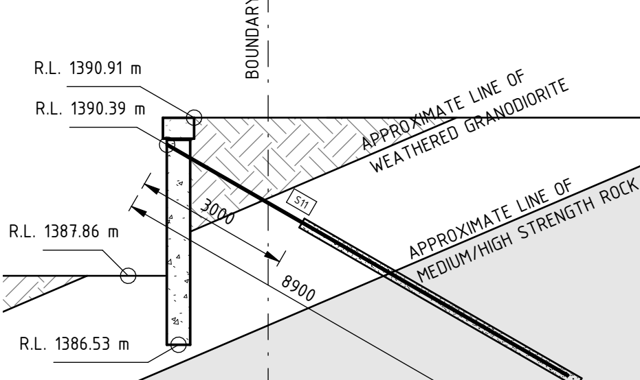
PILE S11
