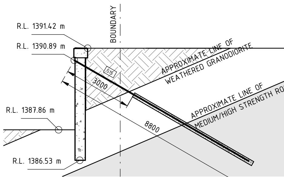
PILE S15
