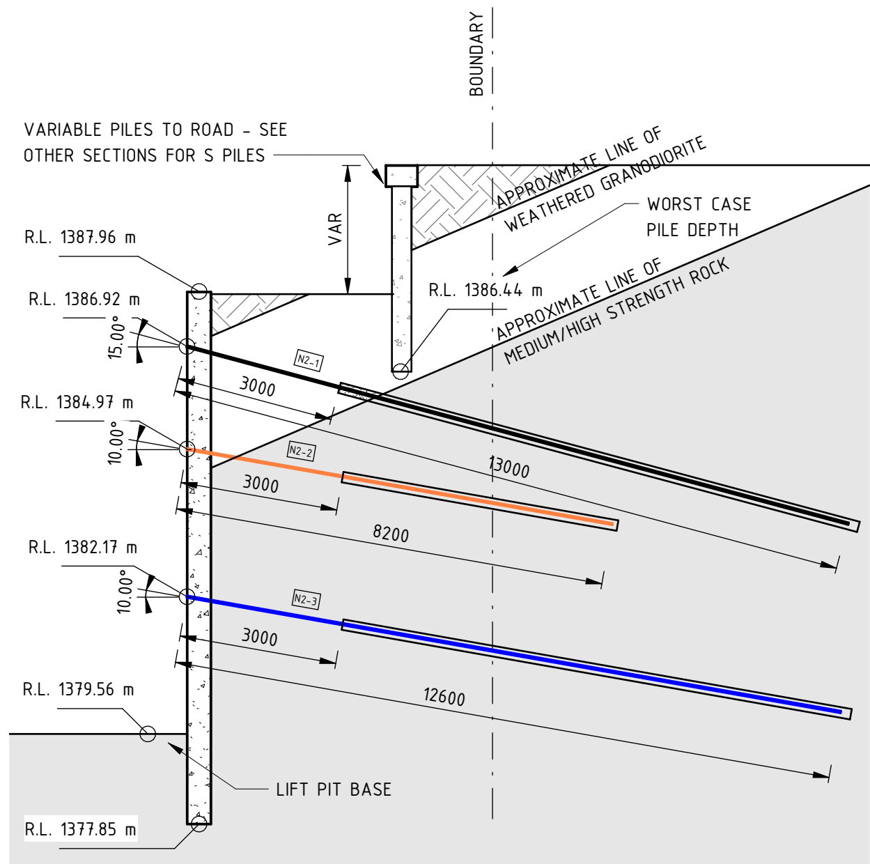
PILES N2
