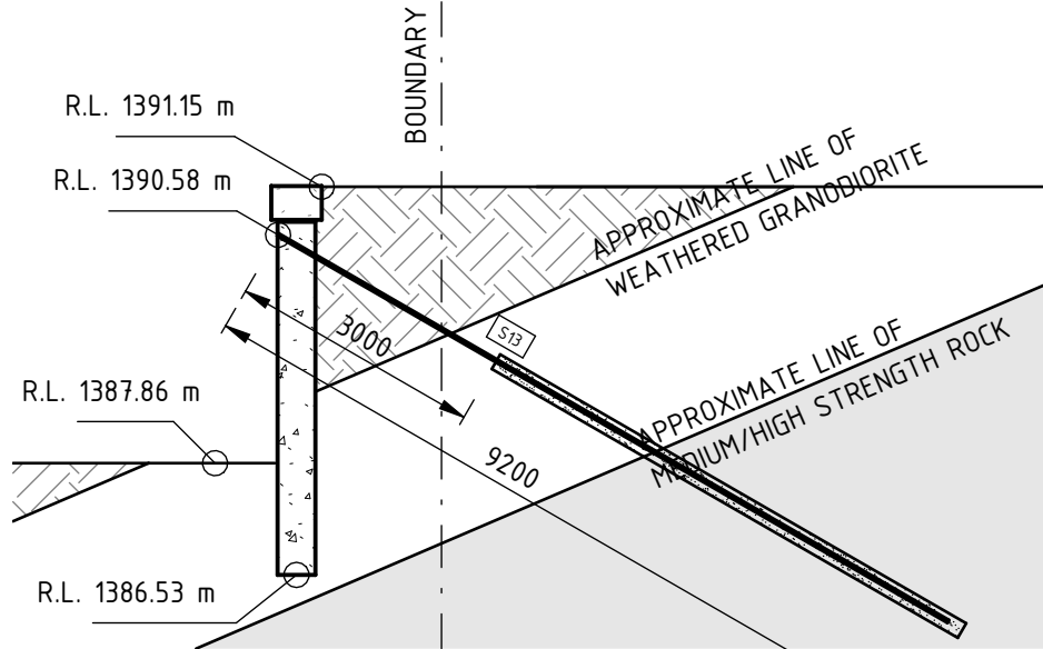
PILE S13
