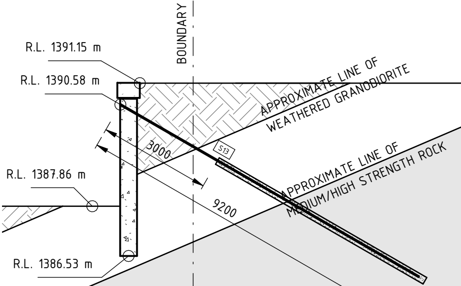
PILE S13
