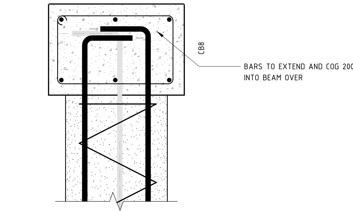
TYPICAL CAPPING BEAM CONNECTION
